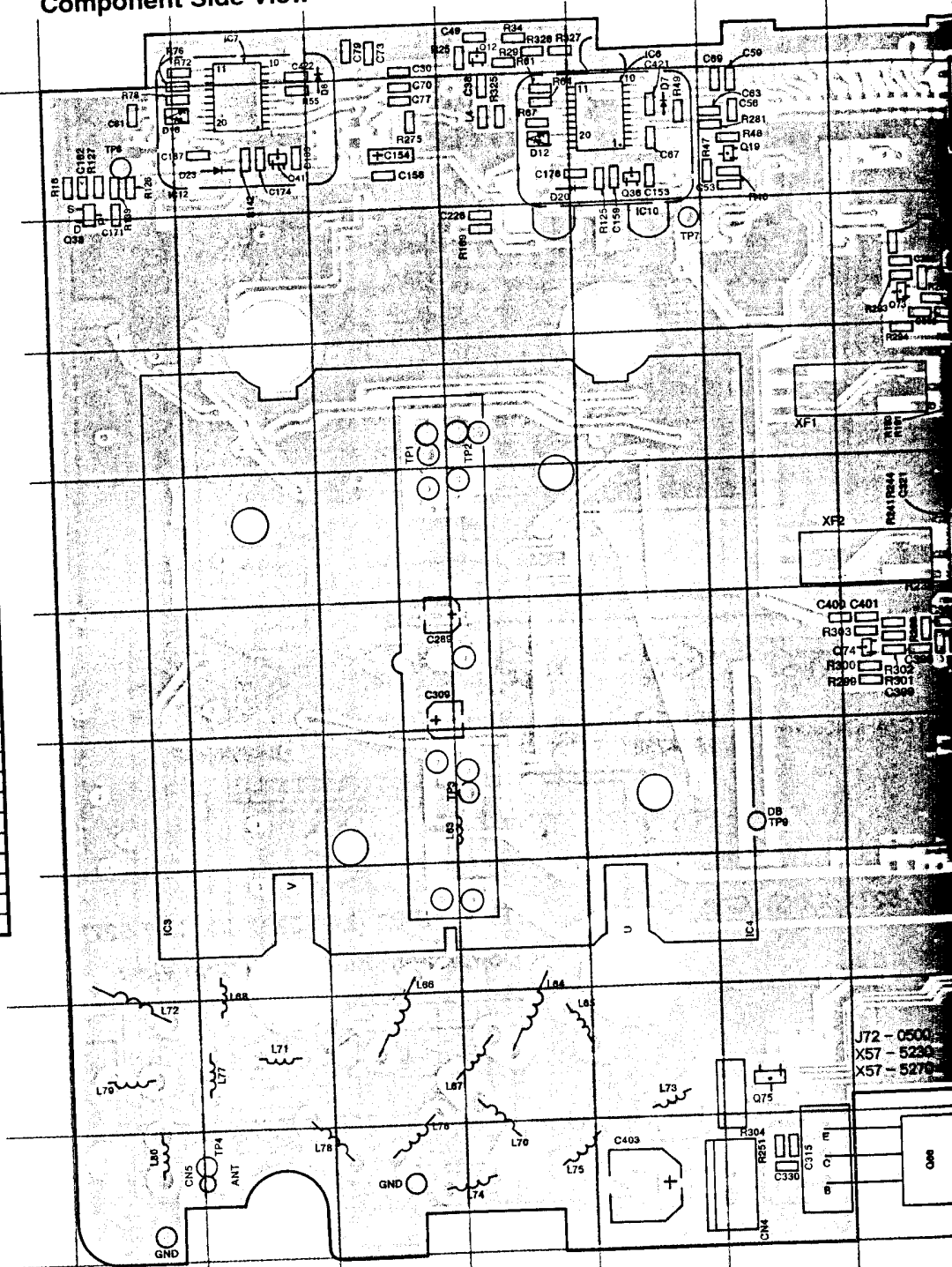
TX-RX UNIT (A/3) (Component side)
