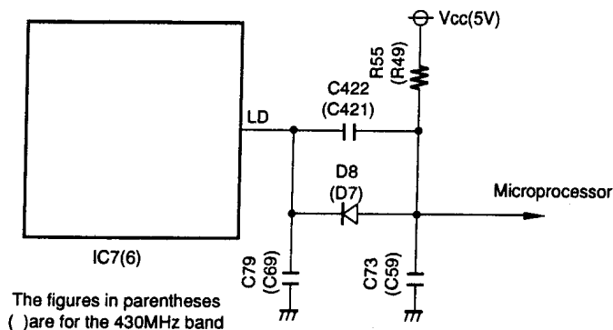
Fig.5 Unlock circuit
