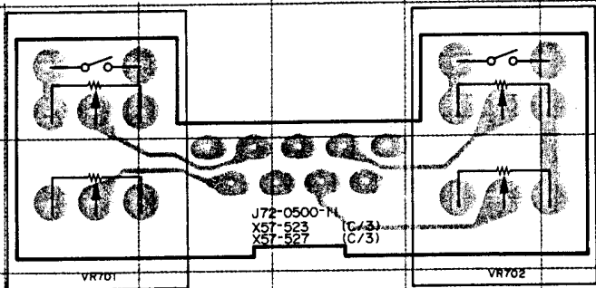
TX-RX UNIT (X57-523X-XX, X57-527X-XX:S) (C/3) Component Side View
