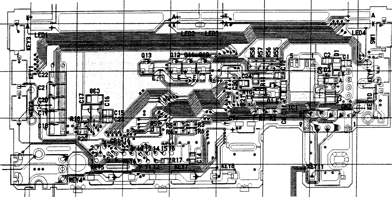
LCD ASSY (B38-0772-15)
