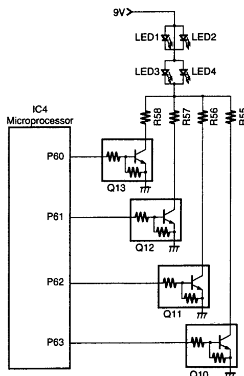
Fig.17 Dimmer circuit
